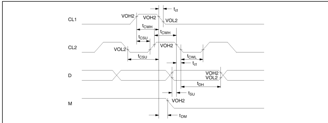
Interface Timing with External Driver
