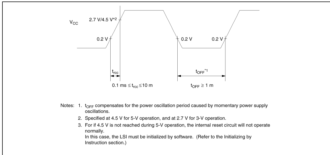
Internal Power Supply Reset
