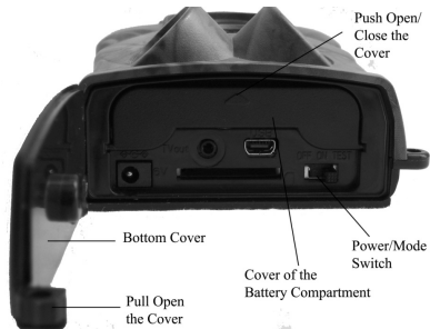
Figure 1.2: Bottom View of Ltl-5310M
